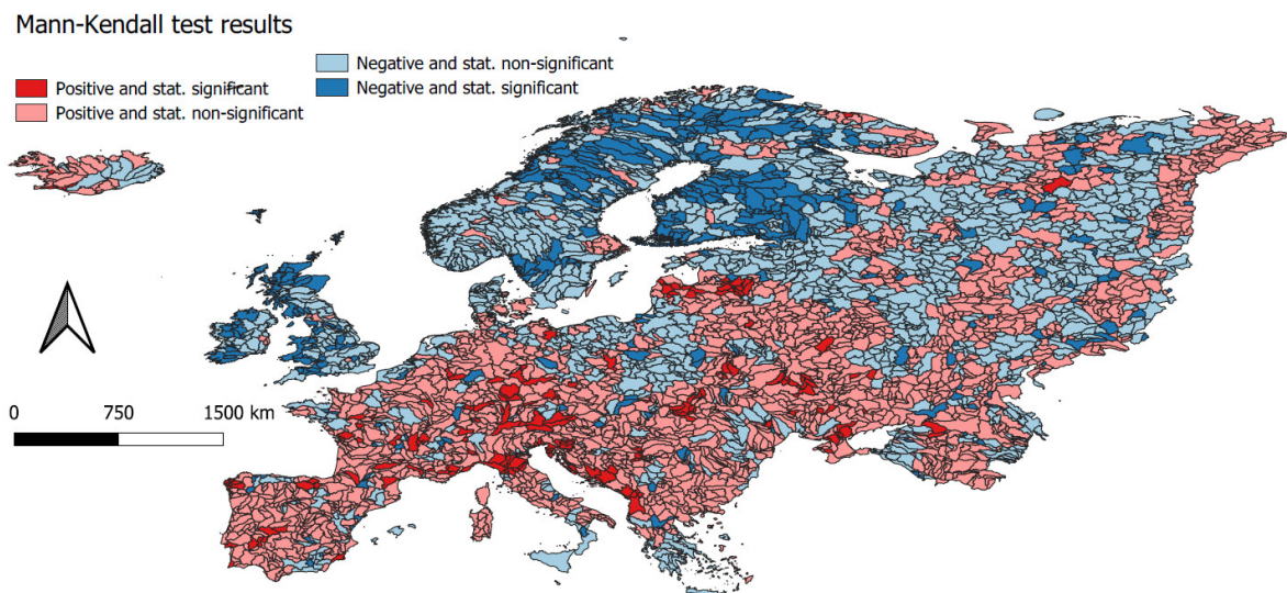
Figure 3. Mann–Kendall trend test results using the mean annual number of days with a compound occurrence of drought and extreme heat in the 1961–2018 period. Results for the basic case and N = 365 days are presented.
