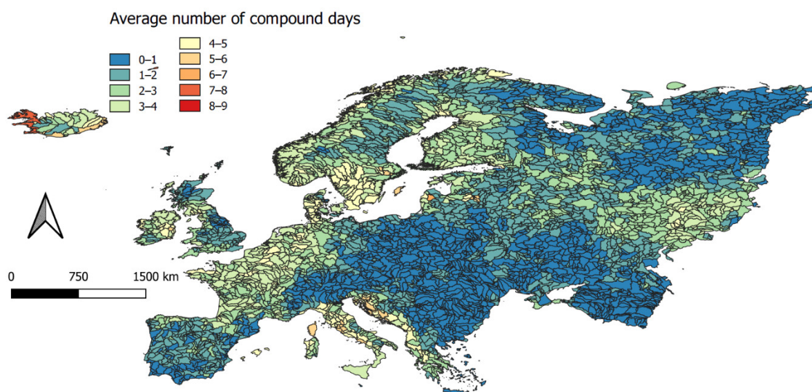
Figure 2. Mean annual number of days with a compound occurrence of drought and extreme heat according to the basic case and 365 days used as the antecedent precipitation ( N ).
