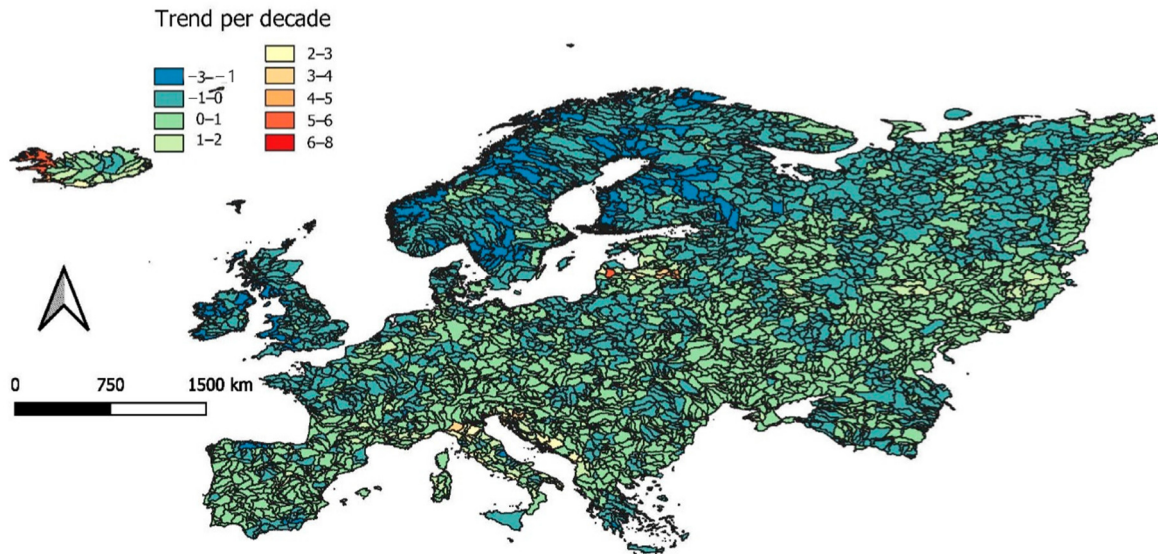
Figure 4. Changes in the mean annual number of days with a compound occurrence of drought and extreme heat in the 1961–2018 period. Results for the basic case and N = 365 days are presented.
